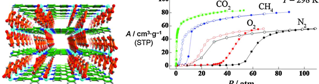
Fig. 11. Structure (left) and gas adsorption/desorption isotherms (right) of Cu(dhbc) 2 (4,4'-bipy).
