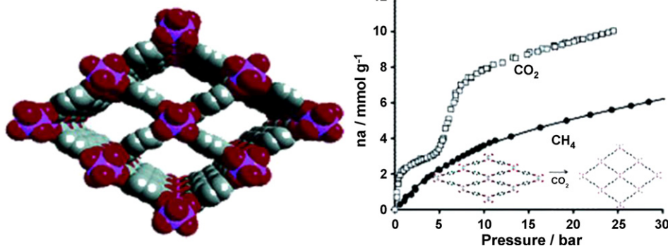
Fig. 23. Structure of MIL-53(Cr) (left) and its CO 2 and CH 4 adsorption isotherms at 304 K (right).
