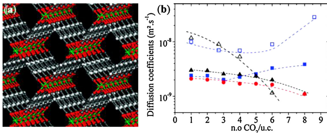
Fig. 9. Structure (a) and the experimental D_o (black \Delta ) and D_t (blue \square ) and the simulated D_s (red \bullet ), D_o (black \blacktriangle ), and D_t (blue \blacksquare ) as a function of CO 2 concentration (b) of MIL-47(V). Reproduced with permission from Ref. [140].
