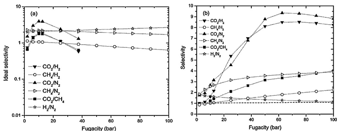
Fig. 20. Predicted (a) ideal and (b) mixture permeation selectivities for a 10 \mu\text{m} thick MOF-5 membrane. The transmembrane pressure drop is 80% of feed pressure. Mixture selectivities are based on an equimolar feed. The first species listed in the labels indicates that permeation of the species that is favored. Reproduced with permission from Ref. [340].
