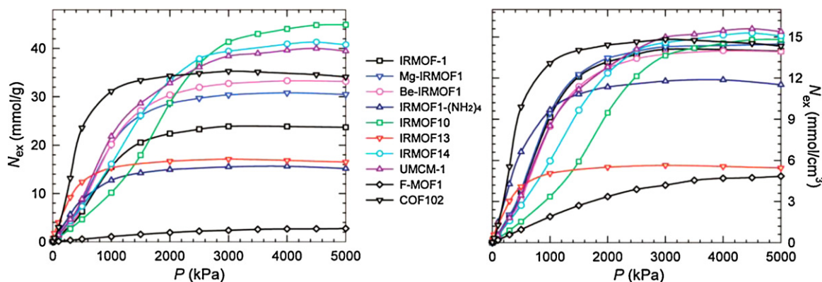
Fig. 19. Gravimetric (left) and volumetric (right) isotherms of CO 2 adsorption in IRMOF1, Mg-IRMOF1, Be-IRMOF1, IRMOF1-(NH 2 ) 4 , IRMOF10, IRMOF13, IRMOF14, UMCM-1, F-MOF1, and COF-102, obtained by GEMC simulations. Reproduced with permission from Ref. [302].
