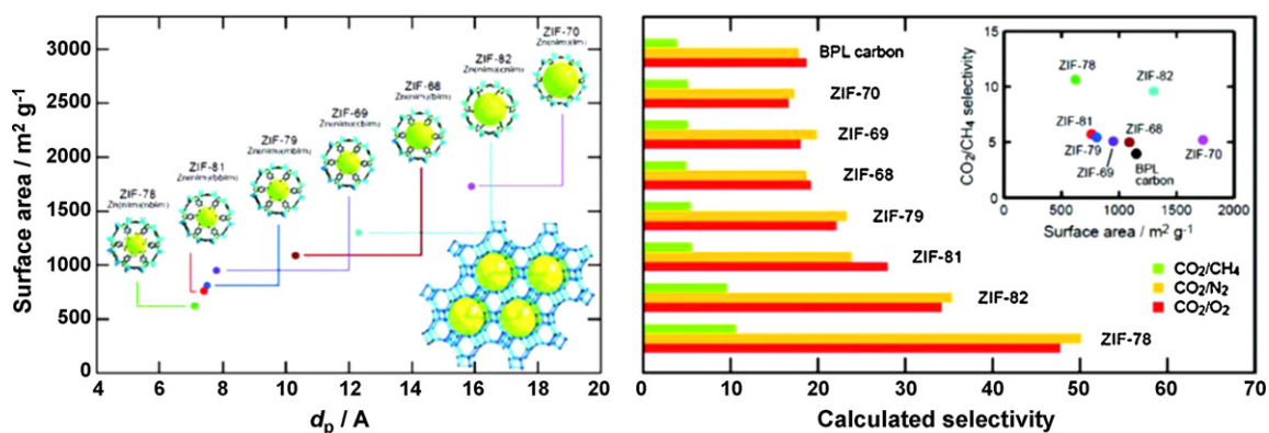
Fig. 21. Plot of pore diameter ( d_p ) vs surface area for different GME ZIFs (left) and the evaluated \text{CO}_2/\text{CH}_4 , \text{CO}_2/\text{N}_2 , and \text{CO}_2/\text{O}_2 selectivities in these ZIFs (right). Reproduced with permission from Ref. [157].
