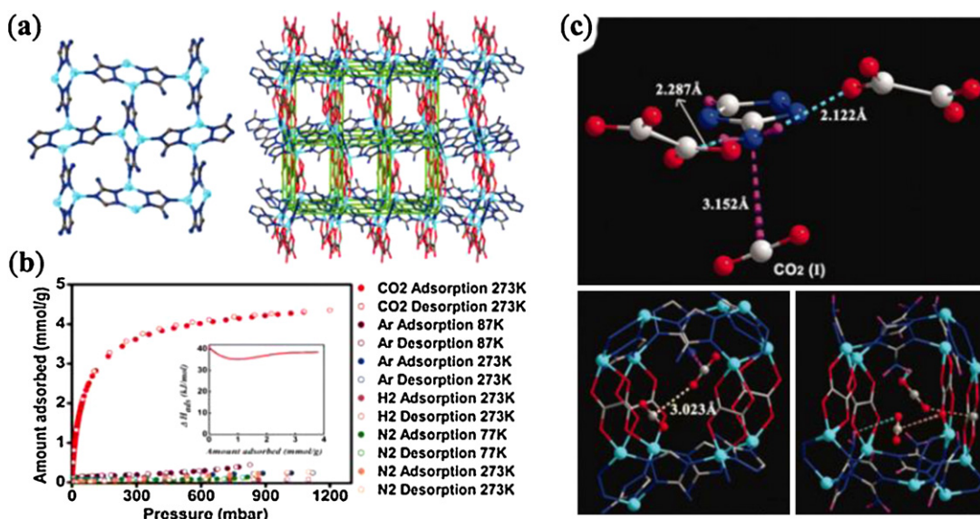
Fig. 7. Structure (a) and gas adsorption properties (b) of Zn_2(ATz)(ox) ; (c) the CO_2 binding (directly determined by X-ray structure refinement at 173 K) within the pores of Zn_2(ATz)(ox) . Reproduced with permission from Ref. [128].
