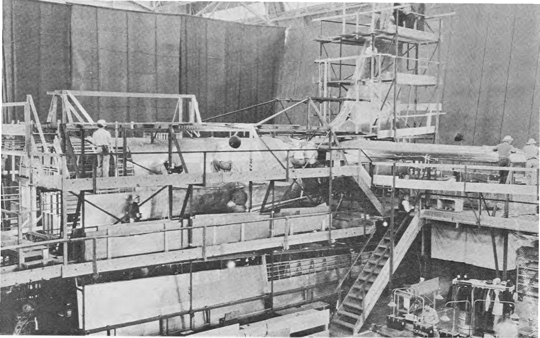
CONSTRUCTION OF EXPERIMENTAL MODEL, DOUGLAS XB-19
