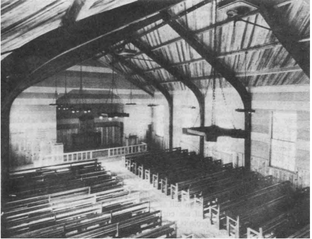
STANDARD CHAPEL (700 SERIES), INTERIOR VIEW
