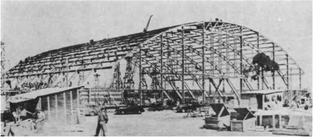
HANGAR CONSTRUCTION, MACDILL FIELD, FLORIDA
