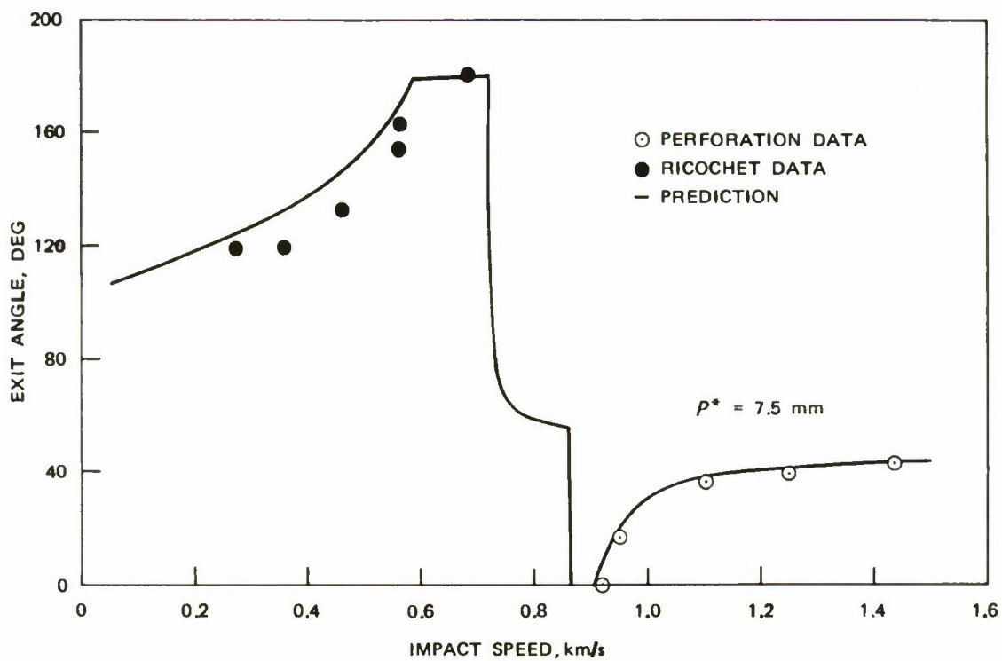
FIGURE 15. Data and Predictions of Exit Obliquities for 6.35-mm Spheres Fired Against 6061 Aluminum Alloy Targets of 9.53-mm Thickness at 45 Degrees Obliquity.
