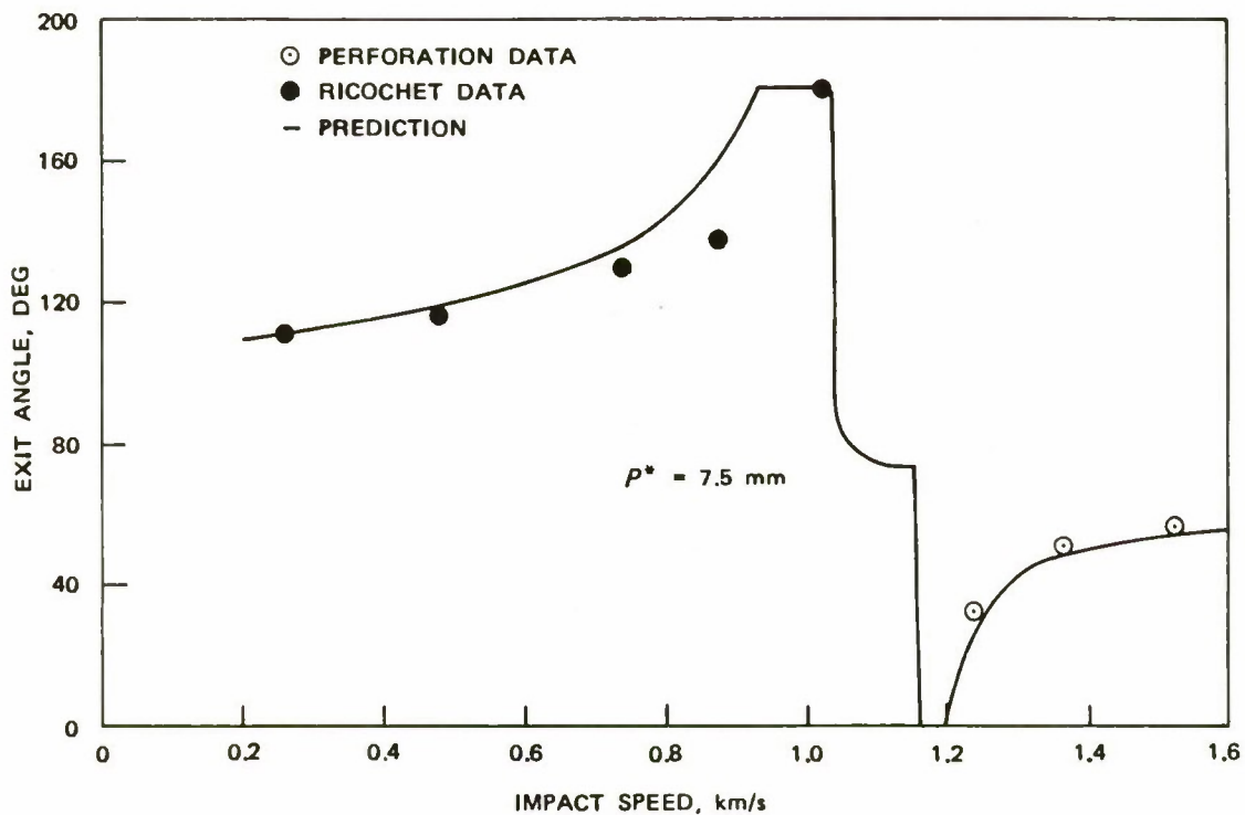
FIGURE 17. Data and Predictions of Exit Obliquities for 6.35-mm Spheres Fired Against 6061 Aluminum Alloy Targets of 9.53-mm Thickness at 60 Degrees Obliquity.
