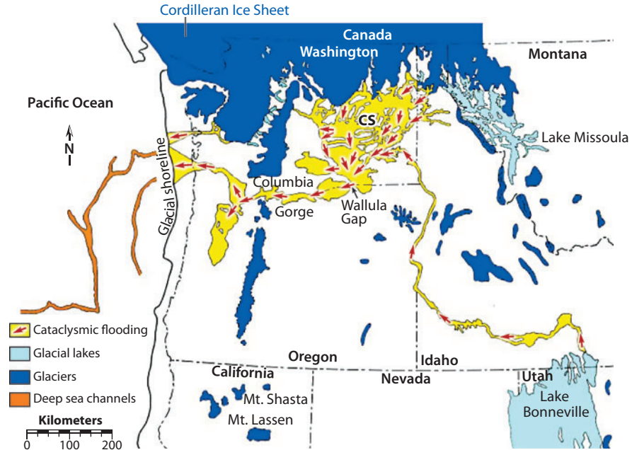
Figure 1 Regions of the northwestern United States affected by late Pleistocene cataclysmic flooding. The Channeled Scabland (CS) is located immediately south of the Cordilleran Ice Sheet and west of glacial Lake Missoula.
