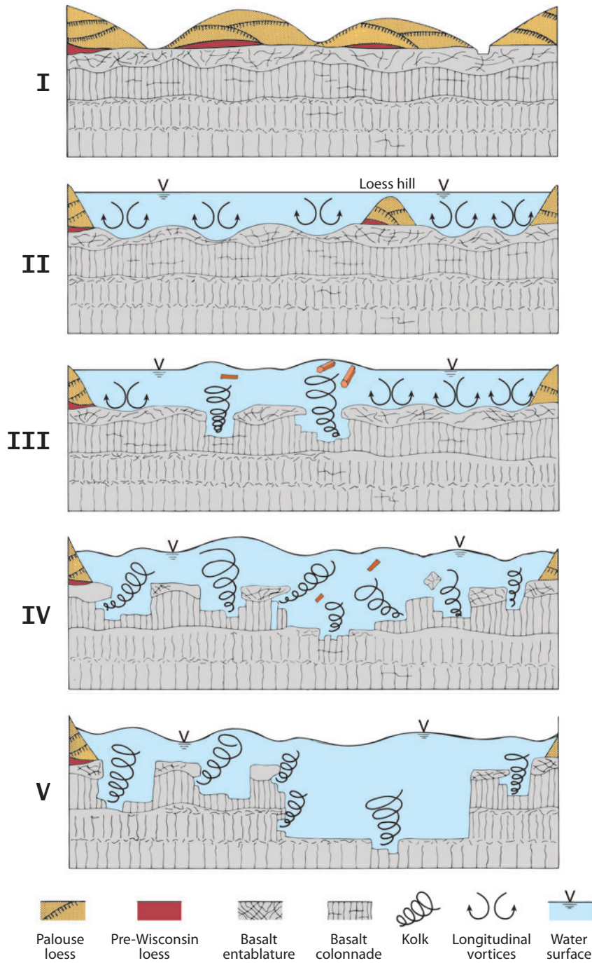
Figure 9 Inferred sequence of erosion for the Channeled Scabland illustrated by schematic cross sections.
