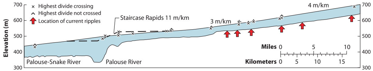
Figure 10 Flow profile along a portion of the Cheney-Palouse scabland tract that shows the use of various high-water marks in reconstructing the paleowater surface during the flooding.
