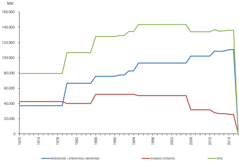
Chart 6.3 – Hydraulic Potential
