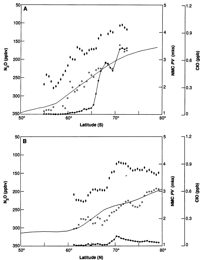
Fig. 4. The structure of the Antarctic (A) and Arctic vortex (B) as observed by high-altitude aircraft near 20 km. The diamonds are measured N_2O averaged into 0.5° latitude and 16 K potential temperature bins. The inside of the vortex is the region poleward of the sharp decrease in N_2O (low values are at the top of the graph). The connected data points show ClO. High abundances of ClO indicate the presence of chemically perturbed air in the vortex. The thin line is potential vorticity derived by the authors from National Meteorological Center gridded global analysis. The small circles show potential vorticity derived from the aircraft data. Potential vorticity is defined as a positive quantity in both hemispheres in these figures.
