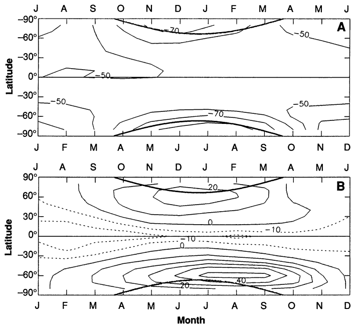
Fig. 3. Time evolution of the temperatures (A) and zonal winds (B) in the lower stratosphere (24 km, 30 mb). Northern Hemisphere data are shifted by 6 months to facilitate comparison. The heavy solid line marks the edge of polar night. Data are from (10).
