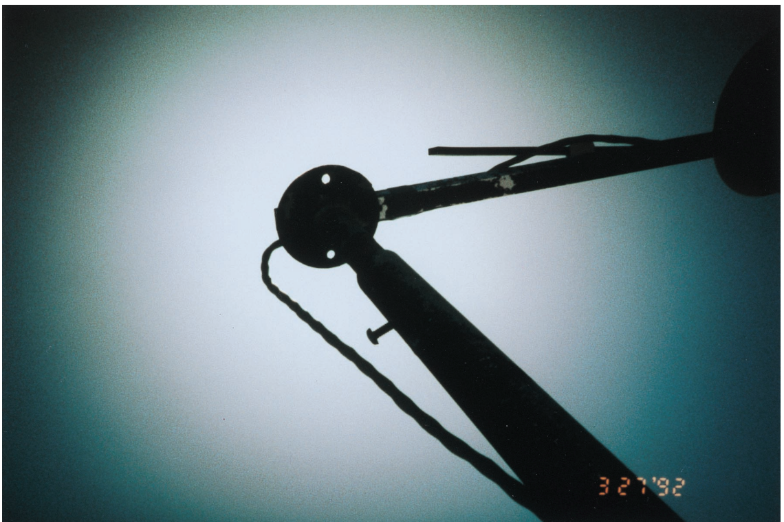
Plate 3. Photograph of sky surrounding the Sun on March 27, 1992, less than 1 year after the Pinatubo eruption, taken at Mauna Loa Observatory by laying the camera on the support shown in Plate 2 and having a portion of that support block out the direct solar radiation. The milky appearance is the enhanced forward scattering (Figure 2), clearly visible to the naked eye. When the stratosphere is clear, the normal appearance is a deep blue produced by molecular Rayleigh scattering. Photograph by A. Robock.
