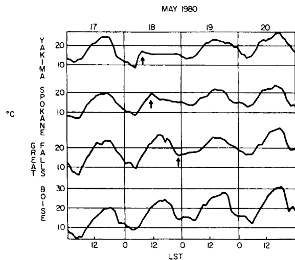
Figure 3. Time series of surface air temperature for Yakima and Spokane, Washington; Great Falls, Montana; and Boise, Idaho, for May 17–20, 1980, under the plume of the 1980 Mount St. Helens eruption, from Figure 3 of Robock and Mass [1982]. Time of arrival of the plume is indicated with an arrow. LST is local standard time. The plume never passed over Boise, which is included as a control. Note the damping of the diurnal cycle after the arrival of the tropospheric aerosol cloud.
