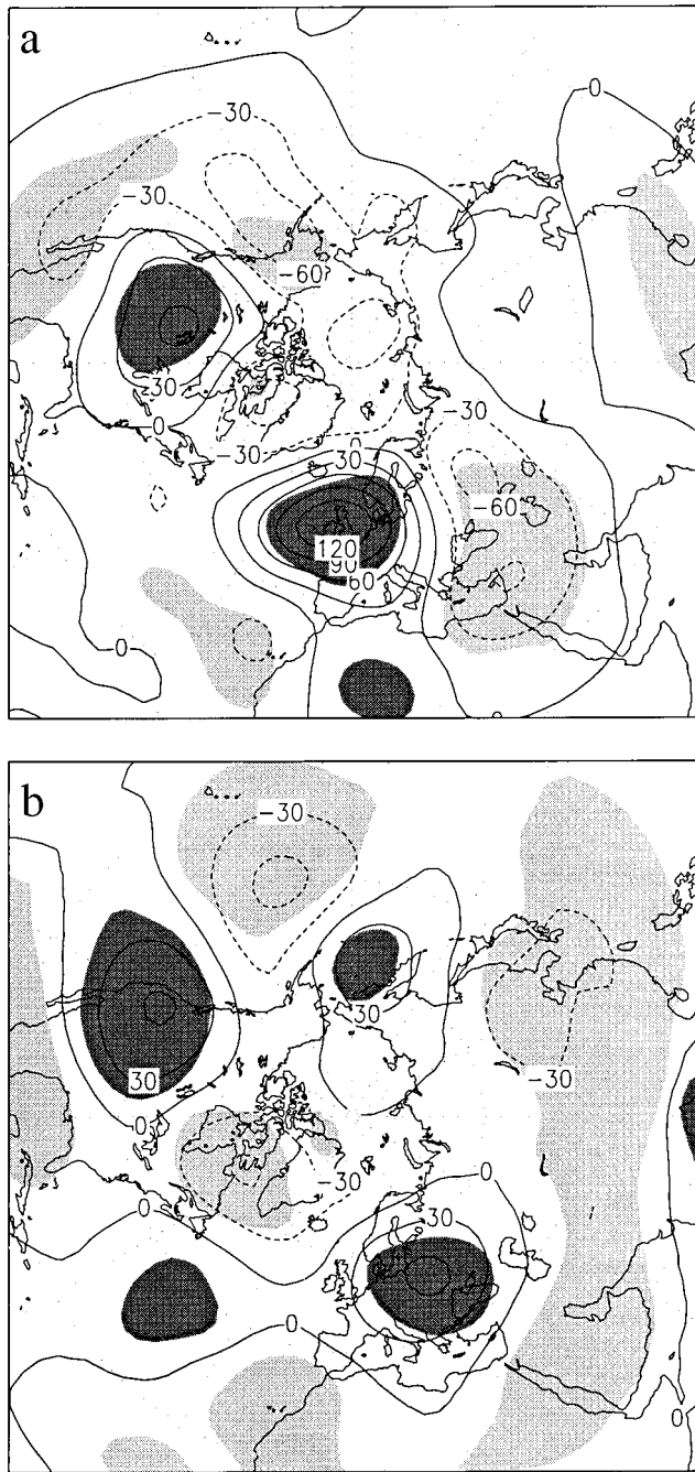
Figure 6. (a) Observed 500-mbar geopotential height (meters) anomaly pattern for the 1991–1992 NH winter (DJF) following the 1991 Mount Pinatubo eruption. Data are from the National Centers for Environmental Prediction reanalysis [Kalnay et al. , 1996], and anomalies are with respect to the period 1986–1990. (b) General circulation model (GCM) simulations from Kirchner et al. [1999]. Shown is the difference between the two GCM ensembles with and without stratospheric aerosols. In both panels, regions significantly different from 0 at the 80% level are shaded, with positive values shaded lighter and negative values shaded darker. The simulations reproduced the observed pattern of circulation anomalies, but not perfectly.
