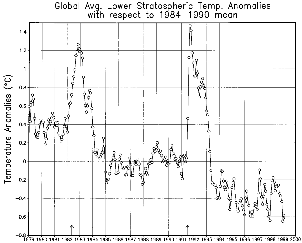
Figure 5. Global average monthly stratospheric temperatures from microwave sounding unit satellite observations, channel 4 [Spencer et al. , 1990] (updated in 1999). Anomalies (°C) are with respect to the 1984–1990 nonvolcanic period. Times of 1982 El Chichón and 1991 Pinatubo eruptions are denoted with arrows. Years on abscissa indicate January of that year.
