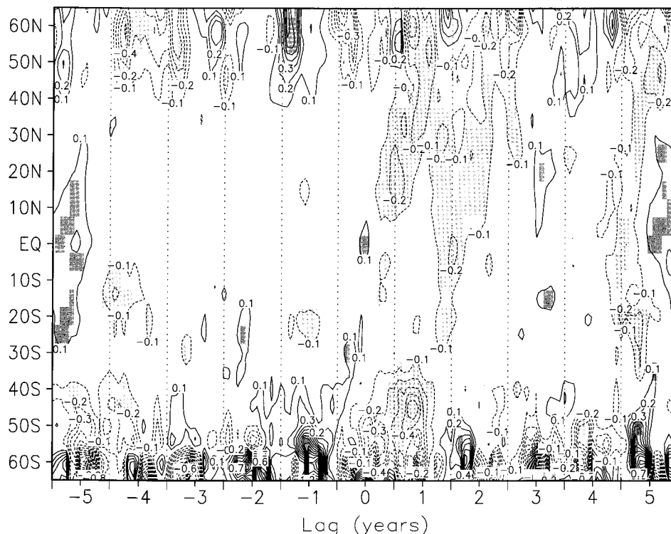
Figure 4. Zonal average surface air temperature anomalies, averaged for the six largest volcanic eruptions of the past century. Anomalies ( ^{\circ}\text{C} ) are with respect to the mean of the 5-year period before each eruption, with the seasonal cycle removed. Values significantly different (95% level) from 0^{\circ}\text{C} are shaded. Contour interval is 0.1^{\circ}\text{C} , with the 0^{\circ}\text{C} interval left out and negative contours dashed. From Figure 6 of Robock and Mao [1995].
