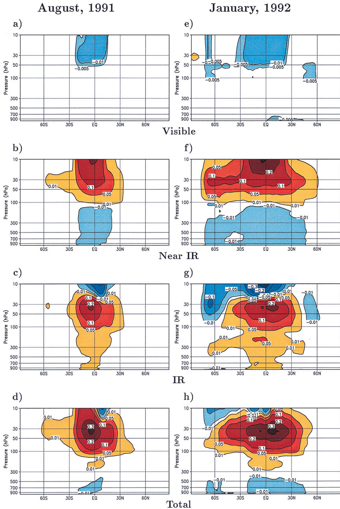
Plate 5. Radiative heating from Pinatubo for three different wavelength bands, from Figure 10 of Stenchikov et al. [1998]. Shown are monthly average, zonal average, perturbations of the radiative heating rates ( K d^{-1} ) caused by the Pinatubo aerosols for (a) visible ( \lambda \leq 0.68 \mu m ), (b) near-IR ( 0.68 \mu m < \lambda < 4 \mu m ), (c) IR ( \lambda \geq 4 \mu m ), and (d) total, for August 1991, and (e) visible, (f) near-IR, (g) IR, and (h) total, for January 1992.
