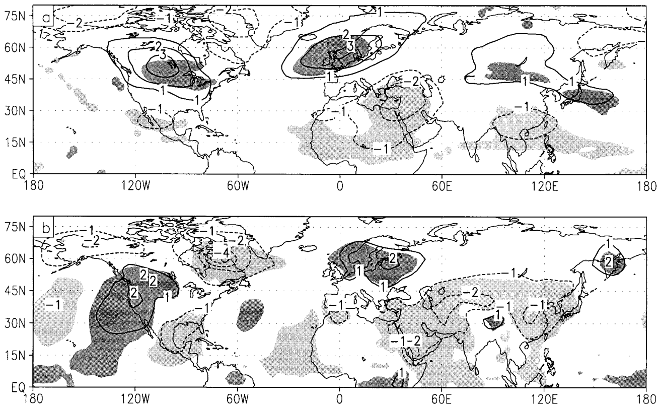
Figure 7. Temperature patterns for NH winter (DJF) 1991–1992 following the Mount Pinatubo eruption. (a) Observed anomalies (with respect to the average for 1986–1990) from channel 2LT of the microwave sounding unit satellite observations (same as in Plate 8), representative of the lower troposphere. (b) Anomalies simulated by a GCM forced with observed Pinatubo aerosols [Kirchner et al. , 1999] expressed as GCM simulated channel 2LT temperatures. Shown are differences between the two GCM ensembles with and without stratospheric aerosols. Contour interval is 1°C, and shading is as in Figure 6. The locations of anomalous warm and cold regions are quite close to those observed.
