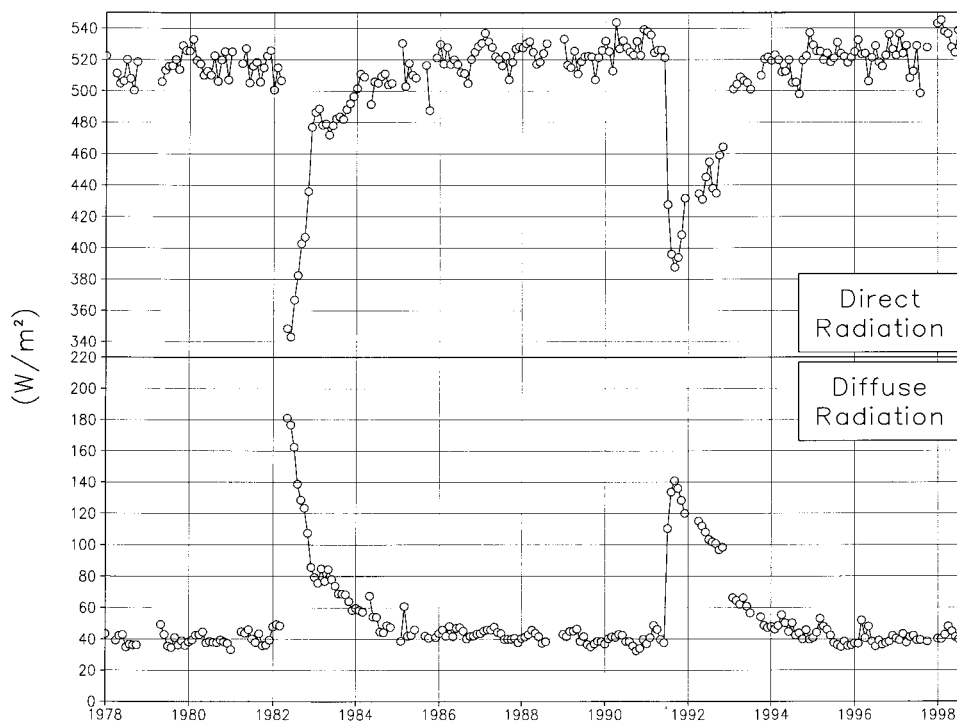
Figure 2. Direct and diffuse broadband radiation measurements from the Mauna Loa observatory, measured with a tracking pyrhelimeter and shade disk pyranometer on mornings with clear skies at solar zenith angle of 60^\circ , equivalent to two relative air masses [Dutton and Christy, 1992]. The reduction of direct radiation and enhancement of diffuse radiation after the 1982 El Chichón and 1991 Pinatubo eruptions are clearly seen. Years on abscissa indicate January of that year. Data courtesy of E. Dutton.
