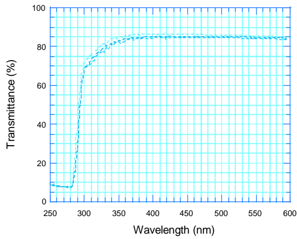
Fig. 2.7 Transmittance of Cover Layer
