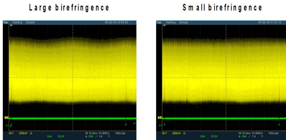
Fig. 2.3 RF envelope variation by birefringence
