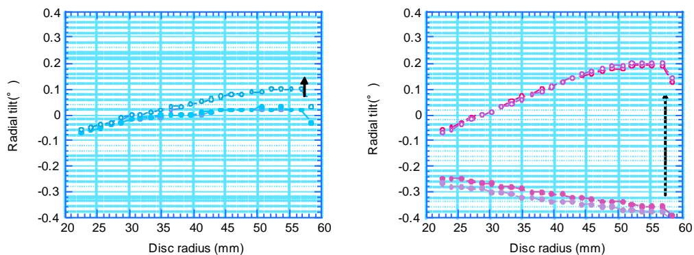
Fig. 2.4 Aging of disc tilt
