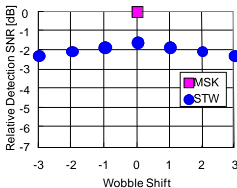
Calculated Signal-to-Noise Ratio for detection of MSK Marks and the STWs using the circuit of Fig.6.3 in case of no cross talk from adjacent Tracks as a function of Wobble shift.
