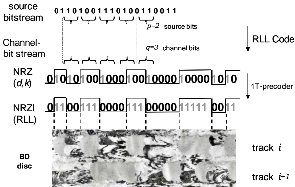
Fig. 5.1.2: RLL d=1 coding for BD optical recording.
