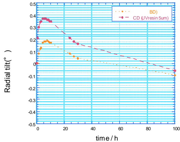
Fig. 2.5 Environmental changes of disc tilt
