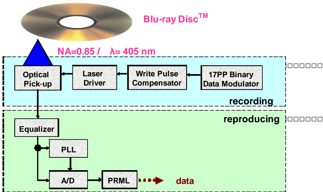
This figure shows a block diagram of Blu-ray Disc™ drive. The 17PP modulated binary data is sent to the Write Pulse Compensator to control the Mark edge position precisely. The output signal of Write Pulse Compensator goes through Laser Driver and Optical Pick-up. The Optical Pick-up has a spherical aberration compensator to focus on the both Layers of the Dual-Layer disc. The reproduced signal was equalized and filtered and passed through PRML decoder to correct the initial bit error.
