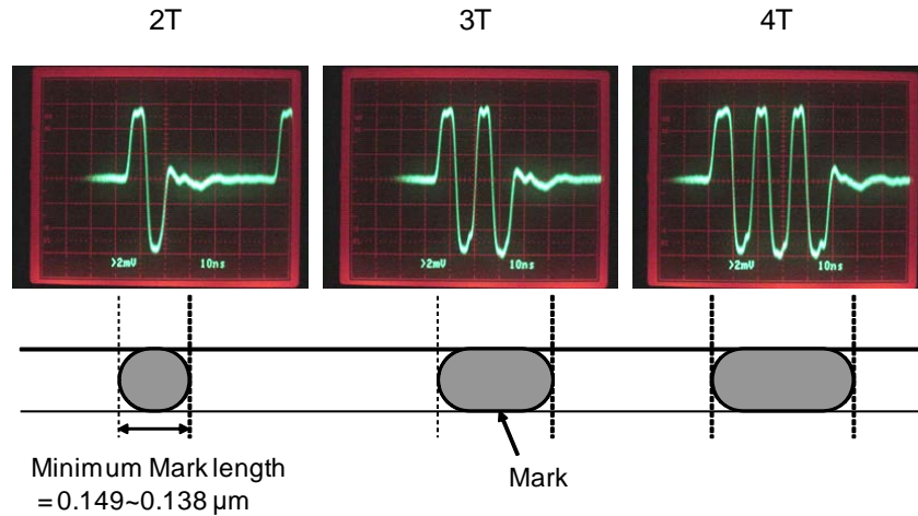
Fig. 3.3.2 Write-pulse waveform
