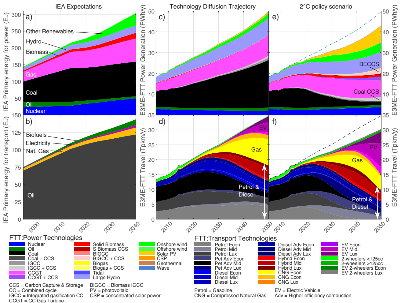
Figure 1 | Projections of future energy use for power generation and transport. a-b) Global IEA fuel demand in the 'IEA expectations' scenario. c-f) Technology composition in electricity generation (c,e) and road transport (d,f) in our 'Technology Diffusion Trajectory' (c-d) and '2°C' scenarios (e-f). IEA fuel demand is taken from [2]. Dashed lines refer to our 'Technology Diffusion Trajectory' scenario for comparison.
