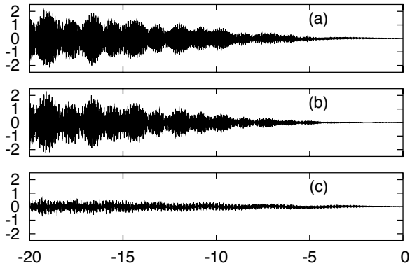
Fig. 7. Differences in obliquity (in degrees) La2004-La93(1,1) versus time (in Myr) over 20 Myr from present (a). In La2004 both orbital and precession model have been changed. In (b) only the precession model has been changed, while in (c) only the orbital motion has been changed. It is thus clear that the main change in La2004 arise from the change of precession model.
