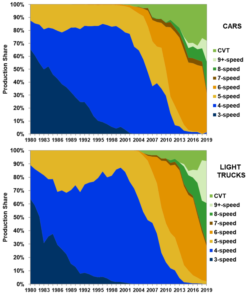
Figure 4.5. Car and Light Truck Production by Transmission Speed, Model Years 1980-2019 (Updated April 2020)
