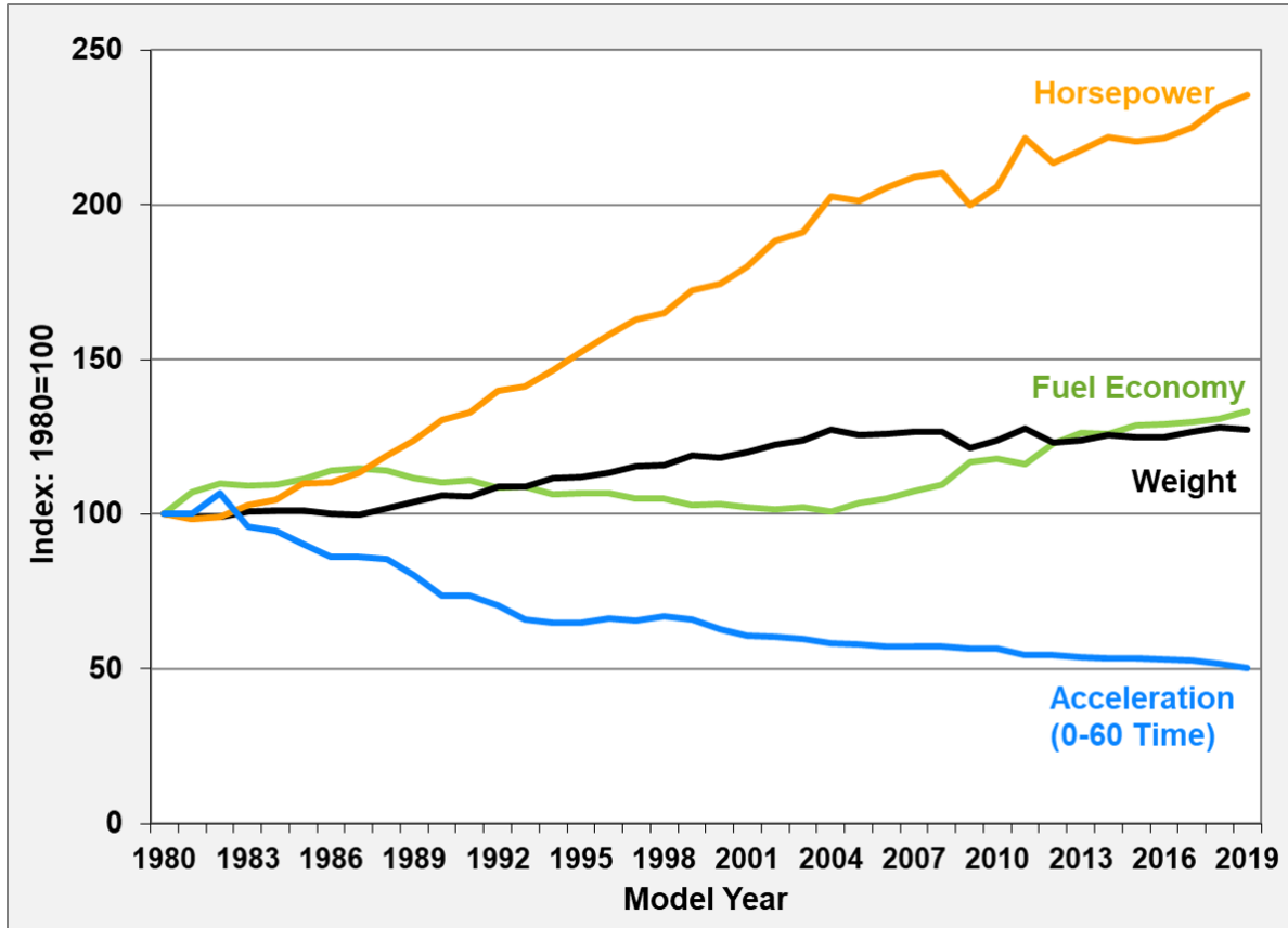
Figure 4.6. Horsepower, Fuel Economy, Weight, and 0-60 Time for New Light Vehicles, Model Years 1980-2019 (Updated April 2020)
