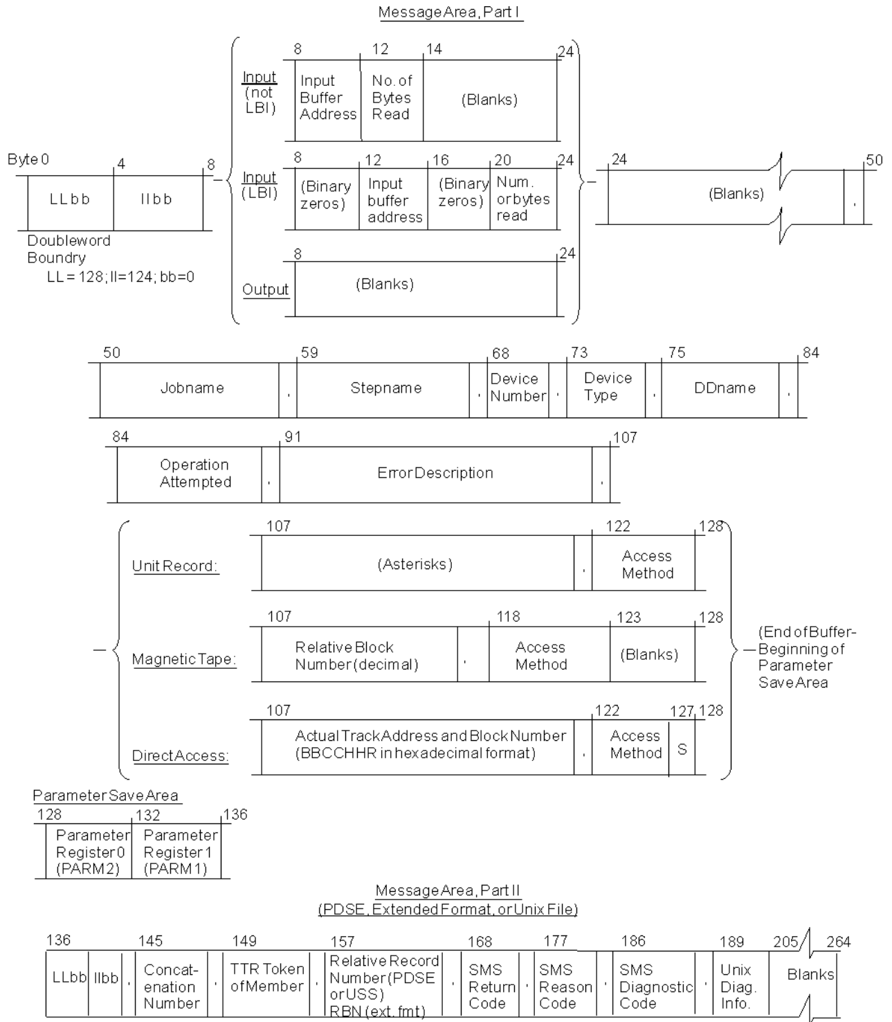
Figure 7: Message Buffer Format
