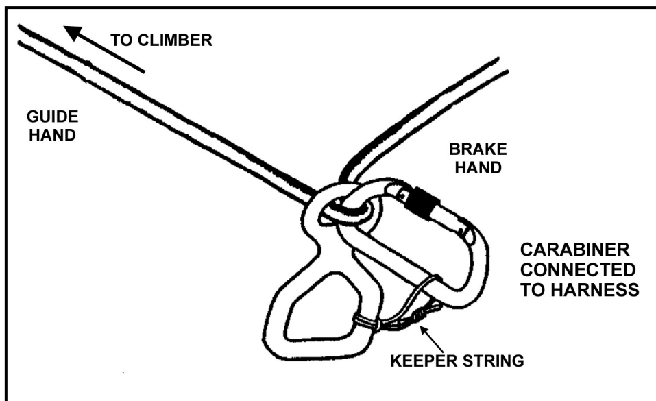
Figure 6-26. Figure-eight device.
