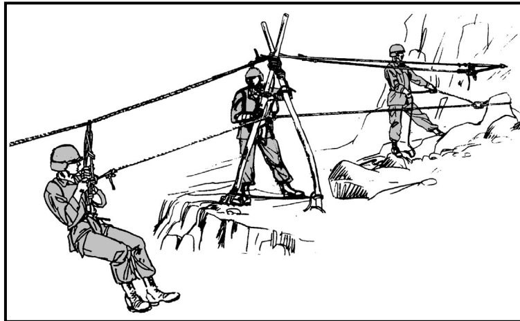
Figure 7-19. Suspension traverse.
