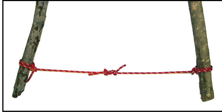
Figure 7-21. A-frame spreader.
