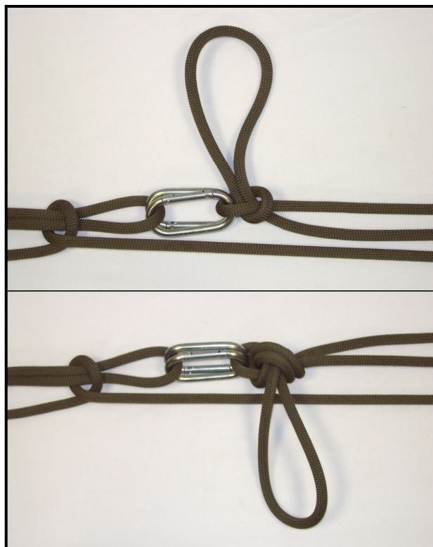
Figure 7-11. Transport knot.
