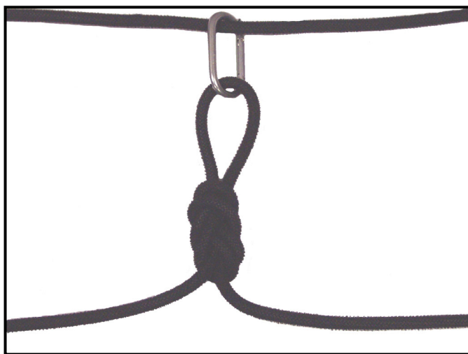
Figure 7-18. Hauling line.
