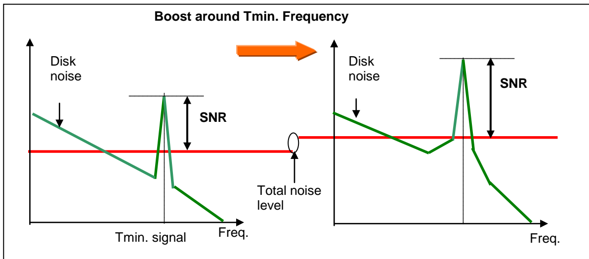
Fig. 1.4.3.1 Improving SNR by boosting high-frequency signal
