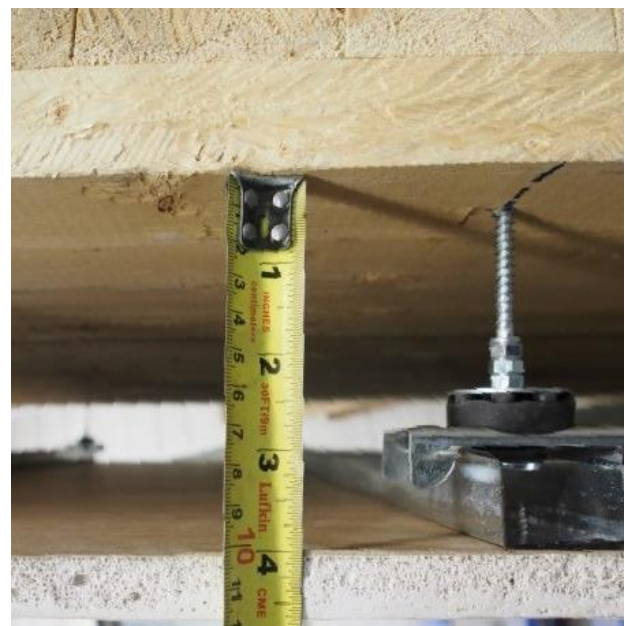
Figure 2: Specimen I-9 with 100 mm cavity
