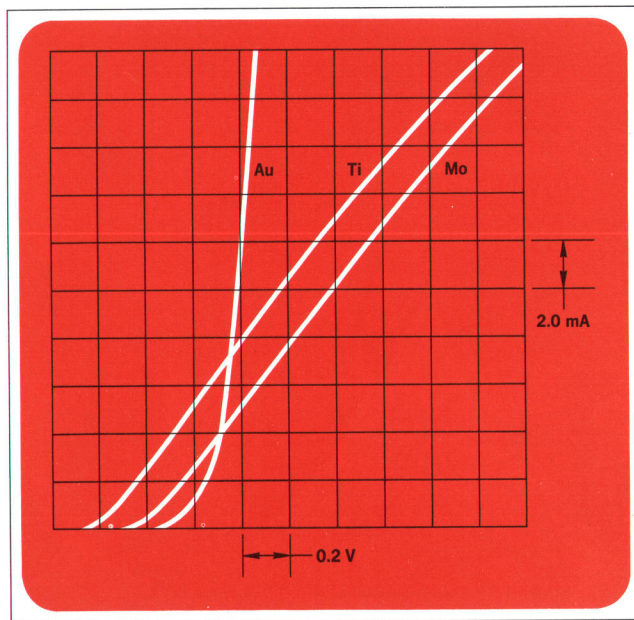
Fig. 8. Au, Mo, and Ti hybrid diode forward I - V characteristics. Diodes were all made on the same silicon wafer. Au diode shows very strikingly the additional current due to hole injection by the p - n junction. This p - n junction current for the Mo and Ti diodes is essentially absent because of the limiting effect of the reverse biased rectifying contact to the diffused ring.
