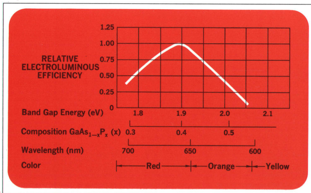
Fig. 6. Red was chosen as the color of the light emitted by the new solid-state indicators because the electro-luminous efficiency of HP's gallium arsenide phosphide alloy is highest for that color. Electroluminous efficiency is a measure of visual brightness per unit diode current. It is a function of the alloy composition, that is, the value of x in the formula GaAs_{1-x}P_x .
