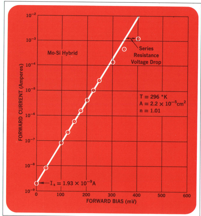
Fig. 5. Forward I-V characteristic of typical Mo-Si hybrid diode conforms closely to theory.
