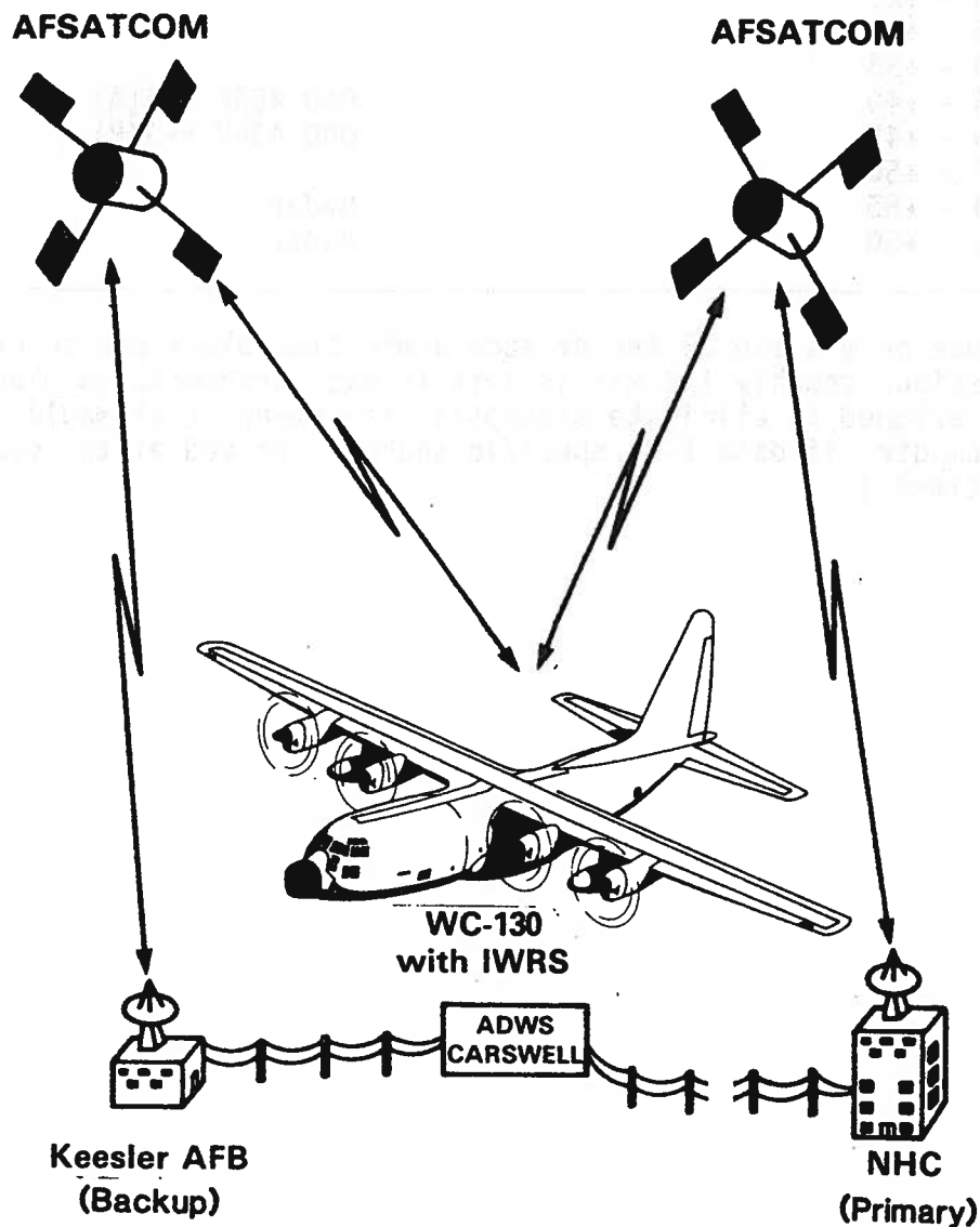
Figure 5-11. Schematic of aircraft to satellite data link for USAF WC-130 aircraft
