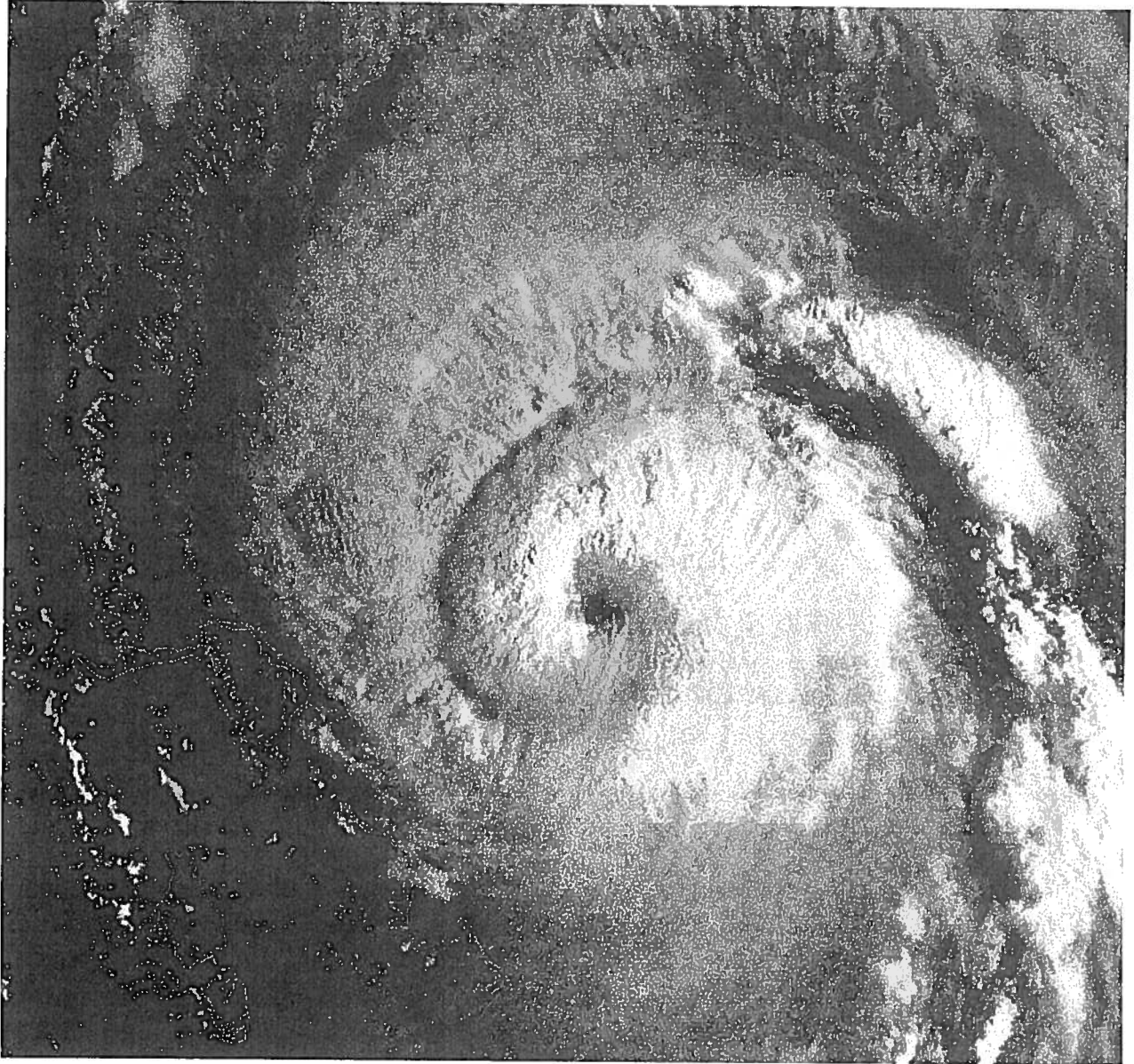
Figure 2-1. Hurricane Fran, September 4, 1996.
