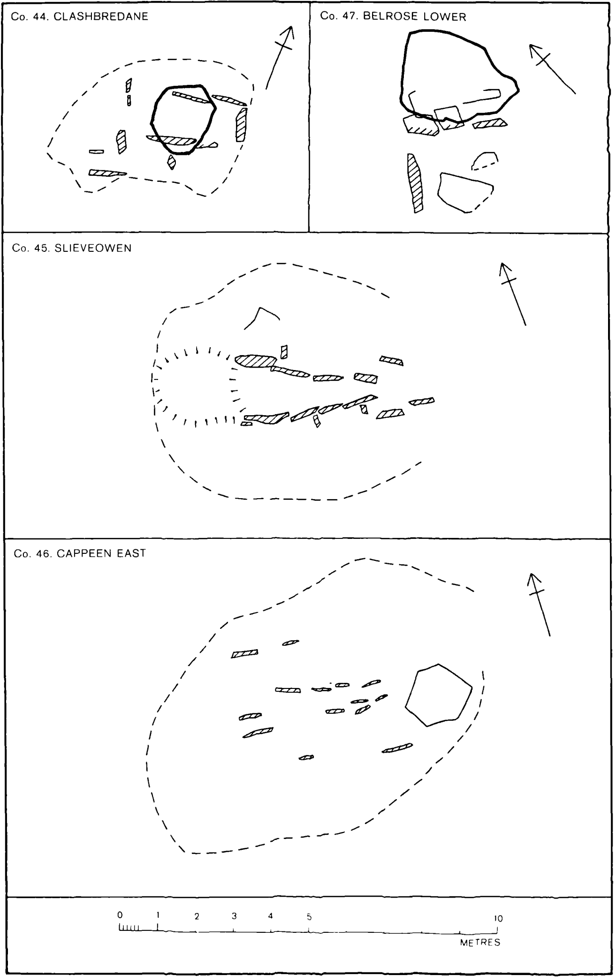
Fig 14 Wedge Tombs Co Cork
