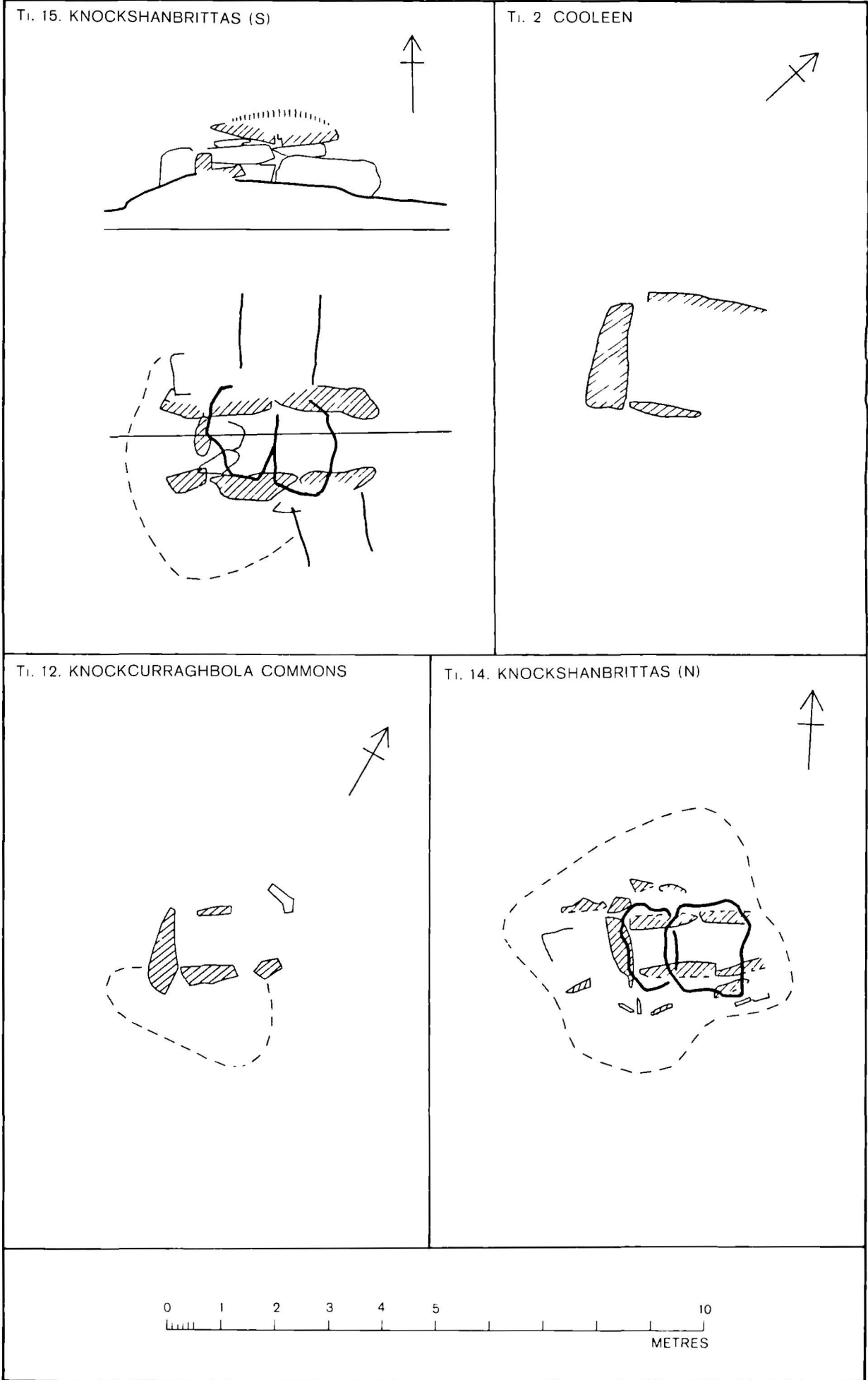
Fig 33 Wedge Tombs Co Tipperary
