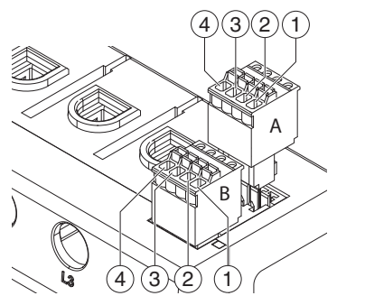
Fig. 3 Connect the RS485 plug
