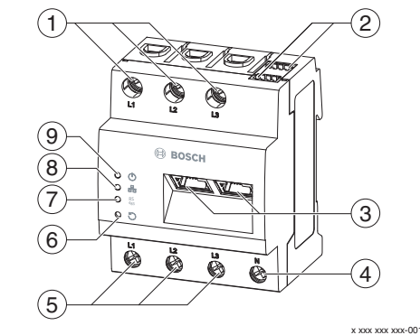
Fig. 1 Product overview
