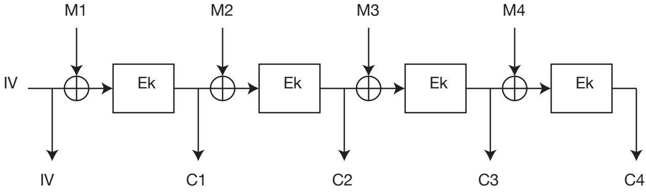
Cipher Block Chaining
