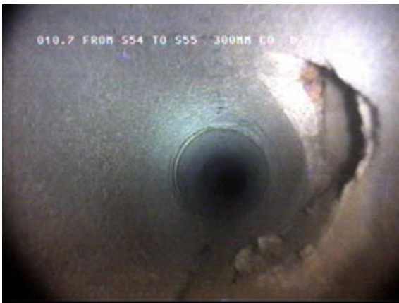
Plate F9 Connection Defect in Pipe
