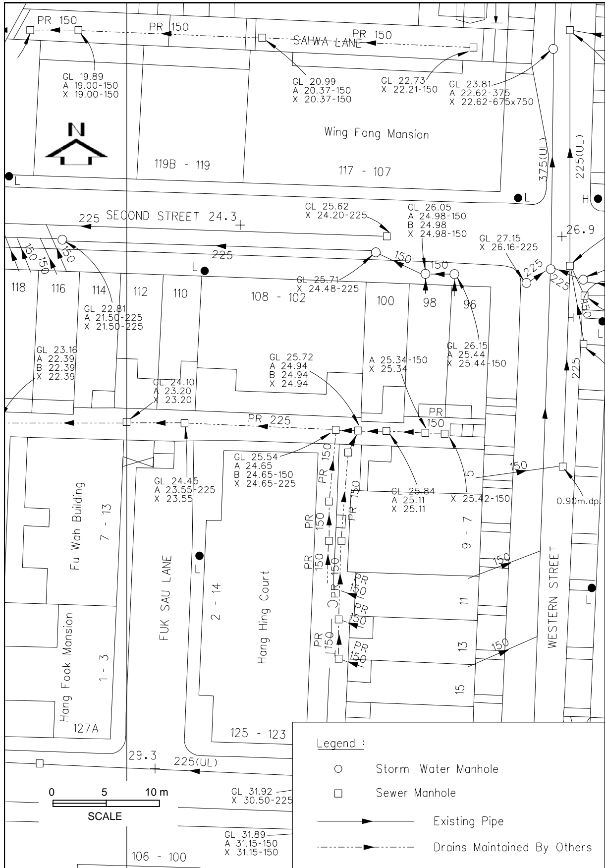
Figure 3.1 Sample As-built Record of Constructed Drains
