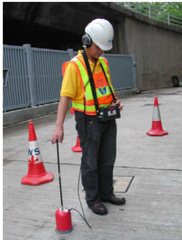
Plate H4 Leak Pinpointing by ELD
