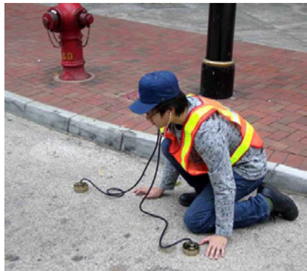
Geophone
