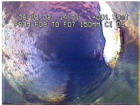
Plate F14 Deposition of Dissolved Salt on Pipe Wall
