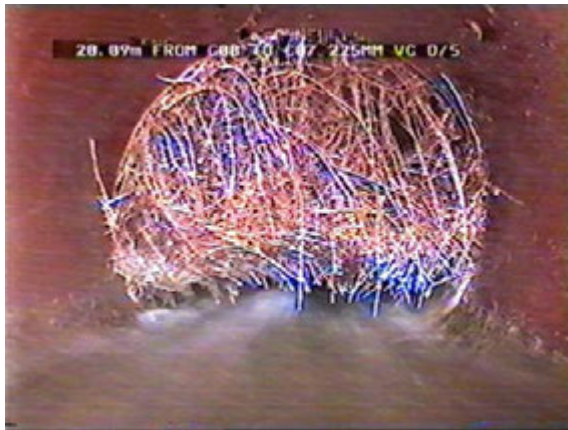
Plate F13 Root Mass Causing Sectional Area Loss
