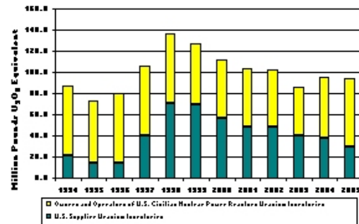
Figure $6. Total Commercial Uranium Inventories of U.S. Suppliers and Owners and Operators of U.S. Civilian Nuclear Power Reactors, 1994-2005
