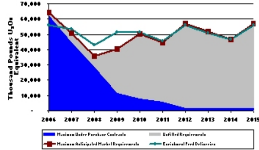
Figure 11. Maximum Anticipated Uranium Market Requirements of Owners and Operators of U.S. Civilian Nuclear Power Reactors, 2006-2015, as of December 31, 2005
