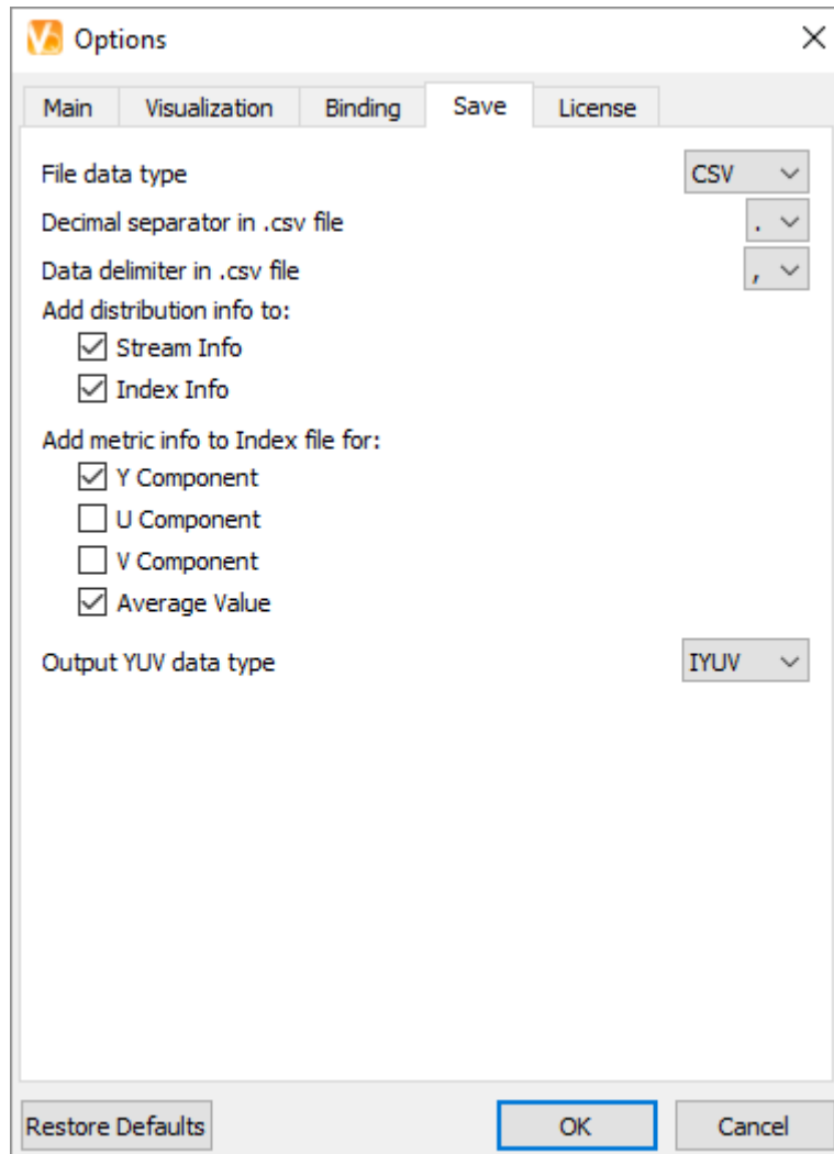
Figure 14. Elecard Video Quality Estimator GUI – Options – Save Tab
