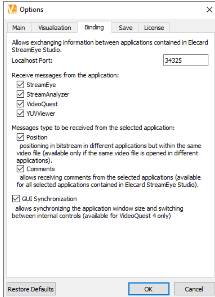
Figure 13. Elecard Video Quality Estimator GUI – Options – Binding Tab
