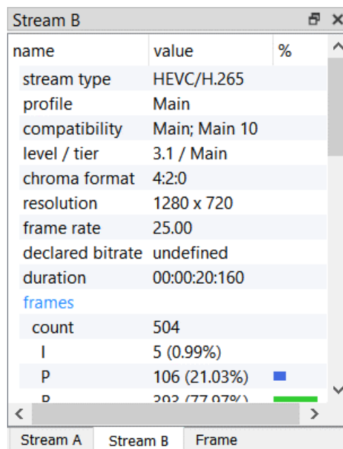
Figure 8. Elecard Video Quality Estimator GUI – Stream Panel
