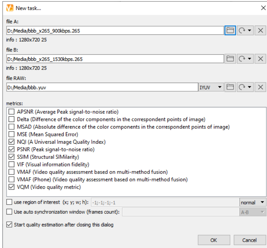
Figure 10. Elecard Video Quality Estimator GUI – New task window
