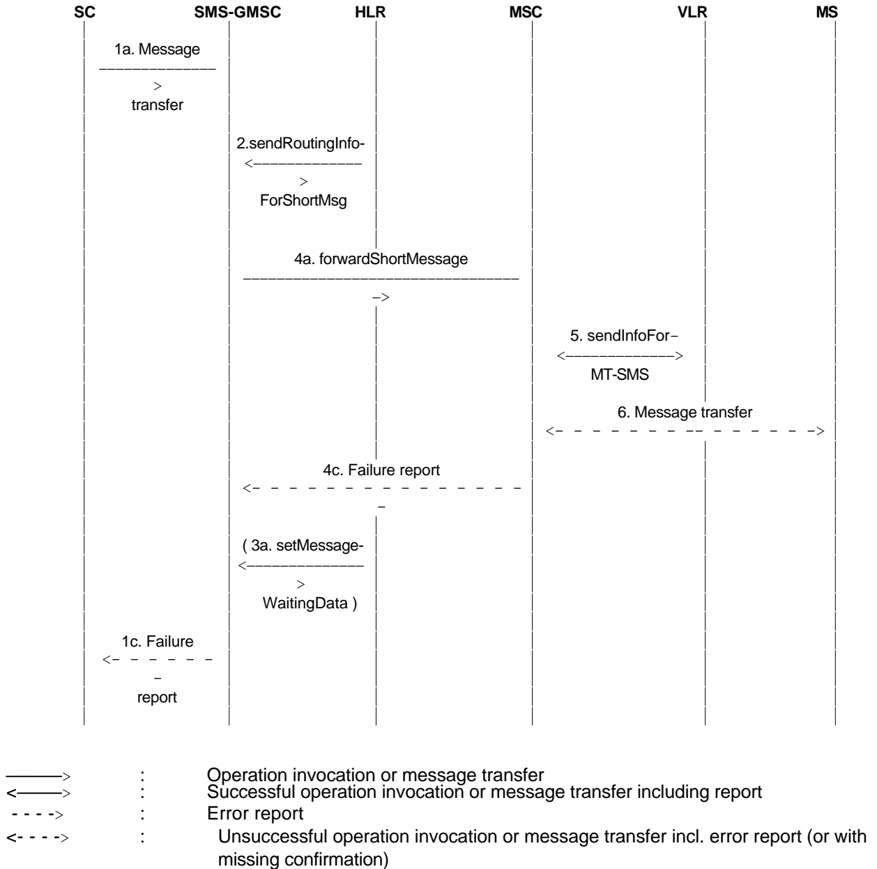
Figure 03.40/15f): Short message transfer attempt failing due to erroneous message transfer on the radio path.
