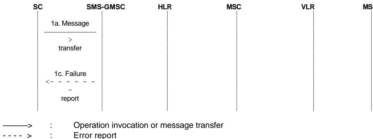
Figure 03.40/15b): Short message transfer attempt failing due to error at the SMS-GMSC.
