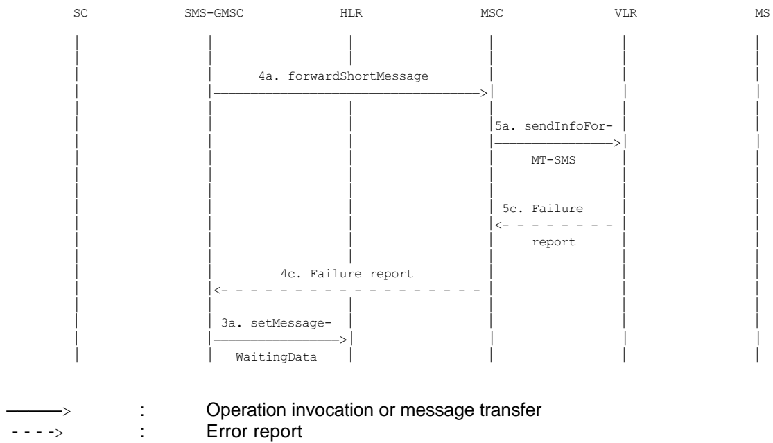
Figure 03.40/16b): 'Send information for MT SMS' procedure; erroneous case: absent subscriber (e.g. IMSI DETACH).
