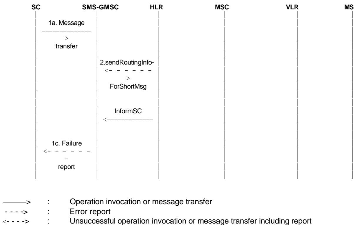
Figure 03.40/15c): Short message transfer attempt failing due to negative outcome of HLR information retrieval.
