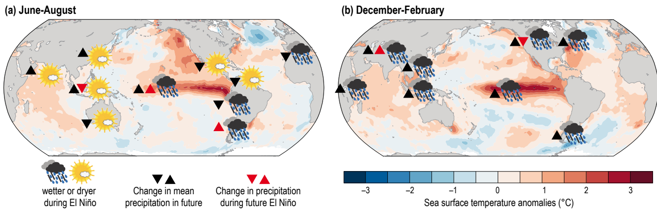
Figure 6.6 | Schematic figure indicating future changes in El Niño teleconnections based on the study of Power and Delage (2018). The background pattern of sea surface temperature (SST) anomalies (°C) are averaged from June 2015 to August 2015 (panel a) and December 2015 to February 2016 (panel b), during the most recent extreme El Niño event (anomalies computed with respect to 1986–2005). Symbols indicate present day teleconnections for El Niño events. Black arrows indicate if there is a model consensus on change in mean rainfall in the region. Red arrows indicate if there is a model consensus on change in the rainfall anomaly under a future El Niño event. Direction of the arrow indicates whether the response in precipitation is increasing (up) or decreasing (down). Significance is determined when two-thirds or more of the models agree on the sign.
