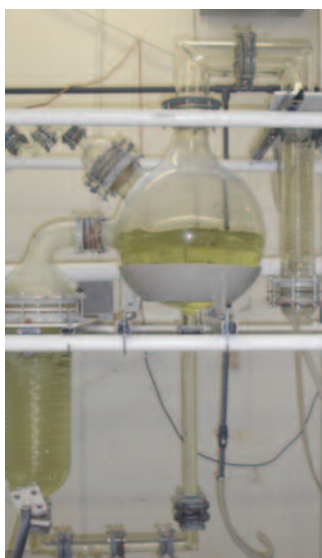
Figure 15: Separation with Heavy Liquids
