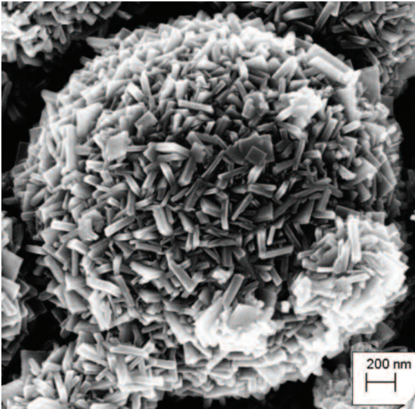
Figure 17: Catalyst Support.
