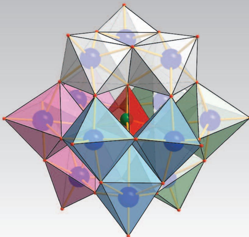
Structure of the Keggin Molecule - Diagram of phosphotungstic acid
