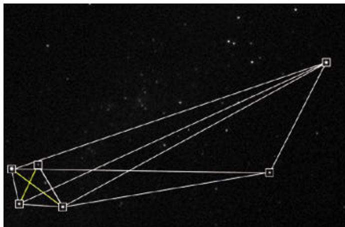
Figure 5. (a) Two Star Tracker Stellar Compasses were used to provide inertial reference for the Clementine satellite. Each Star Tracker weighed only 0.29 kg. (b) This image was taken by the Star Tracker on February 15, 1994, from the Clementine spacecraft during its second loop around Earth prior to lunar orbit. Triangles illustrate how a star match is achieved by comparing the position of detected objects with an on-board database of triangles prebuilt from star positions listed in a whole-sky star catalog. In this case, a match with the Southern Cross constellation, shown in yellow, was achieved.
