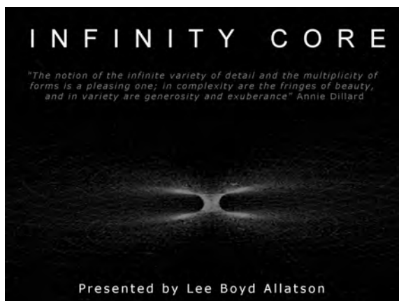
Figure 6. Infinity Core
