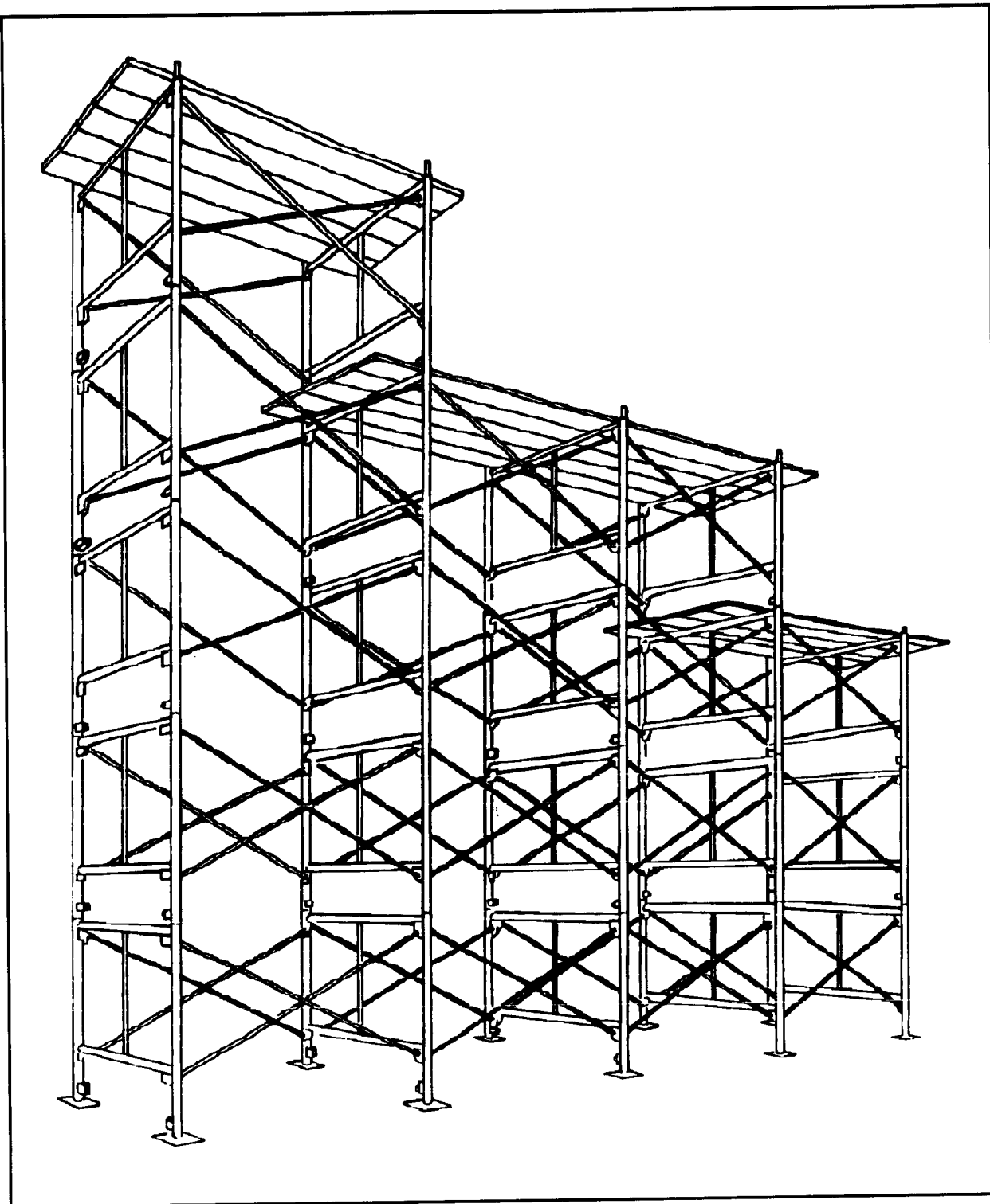
Figure 6-5. Independent scaffolding
