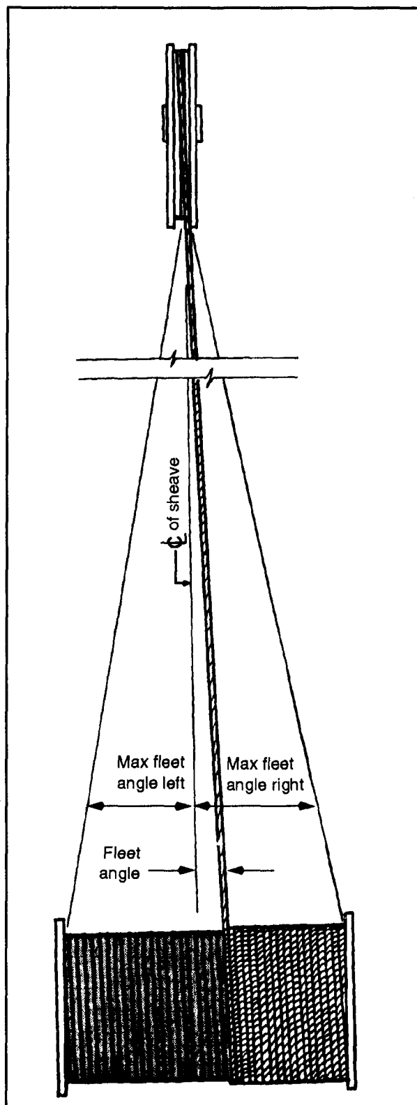
Figure 3-23. Fleet angle
