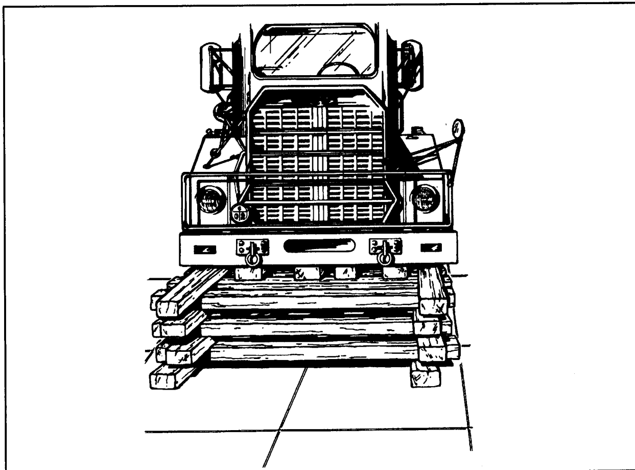
Figure 5-12. Timber cribbing
