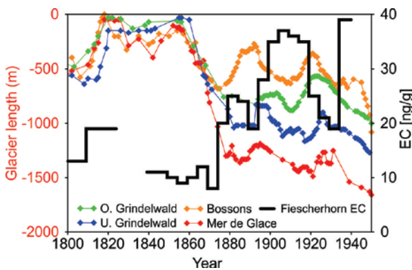
Fig. 1: Low-resolution Fiescherhorn elemental carbon (EC) ice core concentration record [2] superimposed on glacier length variations of the four Alpine glaciers Bosson, Mer de Glace and Oberer Grindelwald between 1800 and 1950 AD [4].
