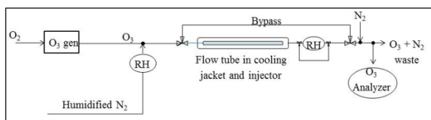
Fig. 1: Schematic of the flow tube experimental setup.
