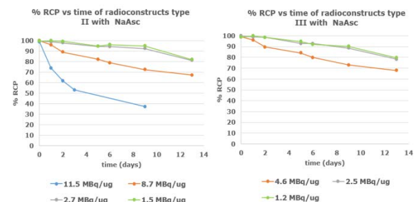
Fig. 4: Radiochemical purity (RCP) vs time of [ ^{177}\text{Lu} ]DOTA-G250 conjugates at 37°C in HSA 1% by ITLC.
