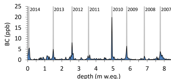
Fig. 3: Dating based on the black carbon concentration signal. Lines indicate Aug./Sept. of each year.
