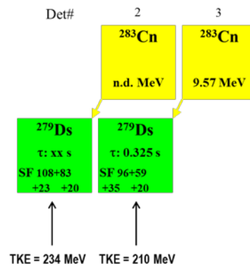
Fig. 2: ^{283}\text{Cn} events observed on the Se-covered detectors #2 and 3, after the target was irradiated with an overall beam dose of 6.30\text{E}+17 ^{48}\text{Ca} particles. No other spontaneous fissions signals were observed. Note the high total kinetic energy of the SF, considering the pulse height defect and gas stopping.
