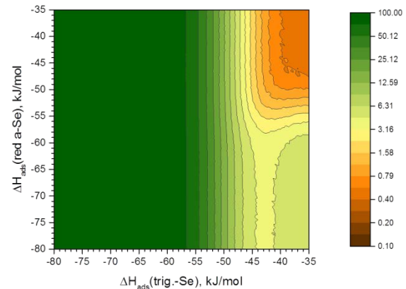
Fig. 3: A preliminary analysis of the probability to observe the two ^{283}\text{Cn} events on the Se-covered detectors, assuming a stationary surface composition on one side of the isothermal part of COLD as 4% red amorphous Se, 80% trigonal Se and 16% \text{SiO}_2 ; The other surfaces of the channel are assumed to consist of \text{SiO}_2 .
