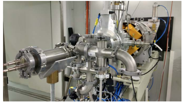
Fig. 2: The BTL equipped with two UniBEaM detectors for x-y beam monitoring followed by the target for the measurements of nuclear excitation functions.
