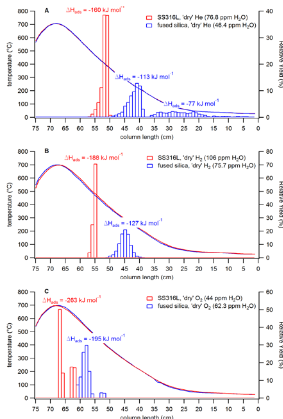
Fig. 1: Thermochromatograms of ^{206}\text{Po} evaporated from LBE heated to 700 °C in SS316L (red bars) and fused silica (blue bars) columns under 'dry' (A) He, (B) \text{H}_2 and (C) \text{O}_2 . The corresponding temperature gradients are shown as color-coded curves. The column material, the carrier gases, and their moisture content in each experiment are indicated.
