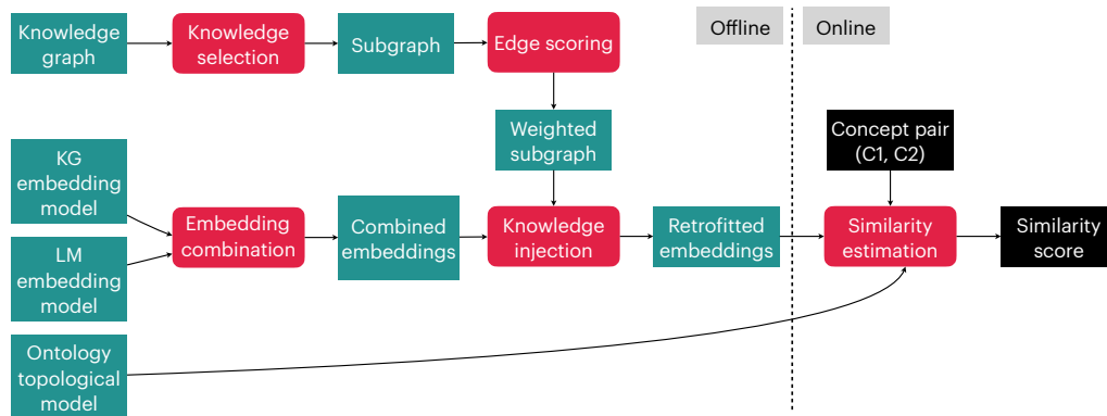
Fig. 2. Overview of our similarity estimation framework.
