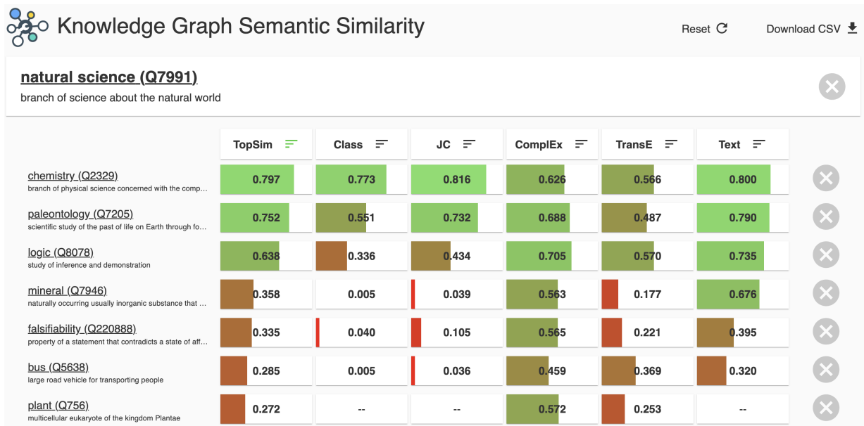
Fig. 1. Example of similarity judgments between natural science and seven other concepts in Wikidata.
