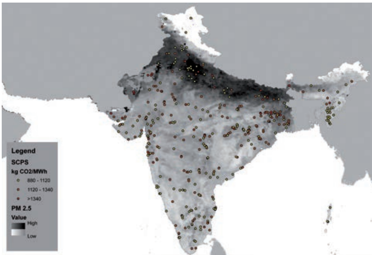
Figure 23: SCPS by Carbon Intensity with PM 2.5 Pollution in India
